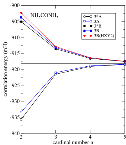
FIG. 1: Convergence of the correlation energy with aug-cc-pV n Z basis sets for NH 2 CONH 2 . The horizontal line indicates the CBS limit, estimated according to the procedure described in the text.
